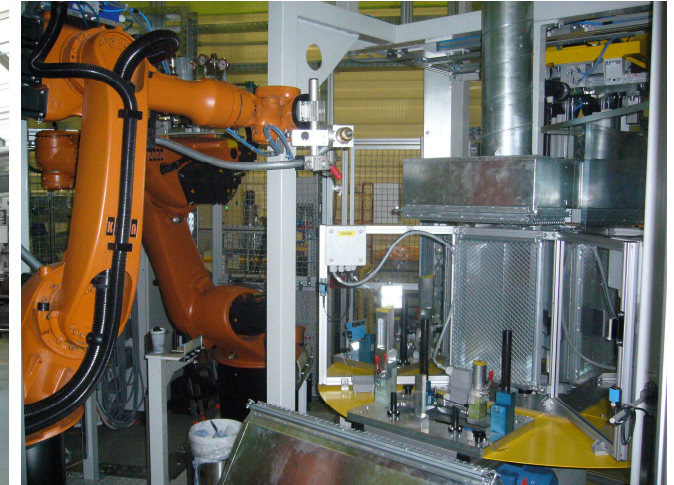
Robot for blowing and plasma
