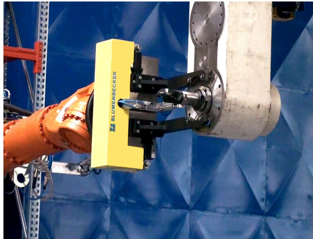
Loading the tool into the spindle of machining center
