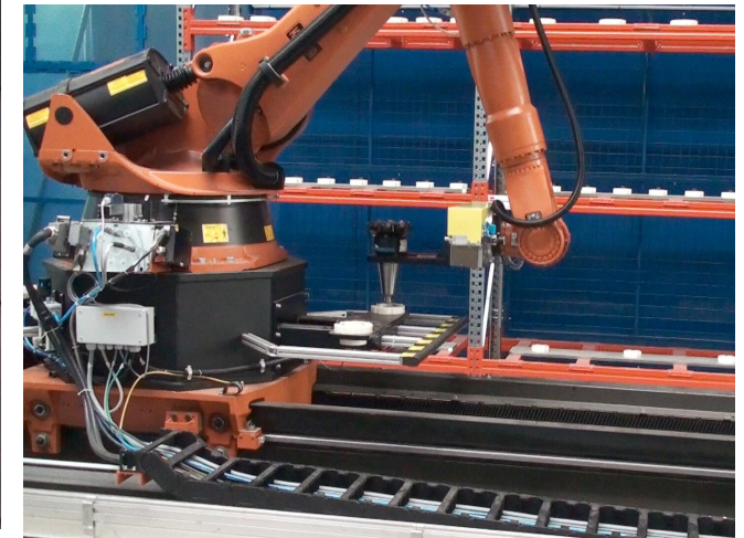
Storing tools in temporary storage on the robot
