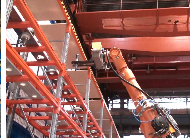
Tools removal from the storage shelf
